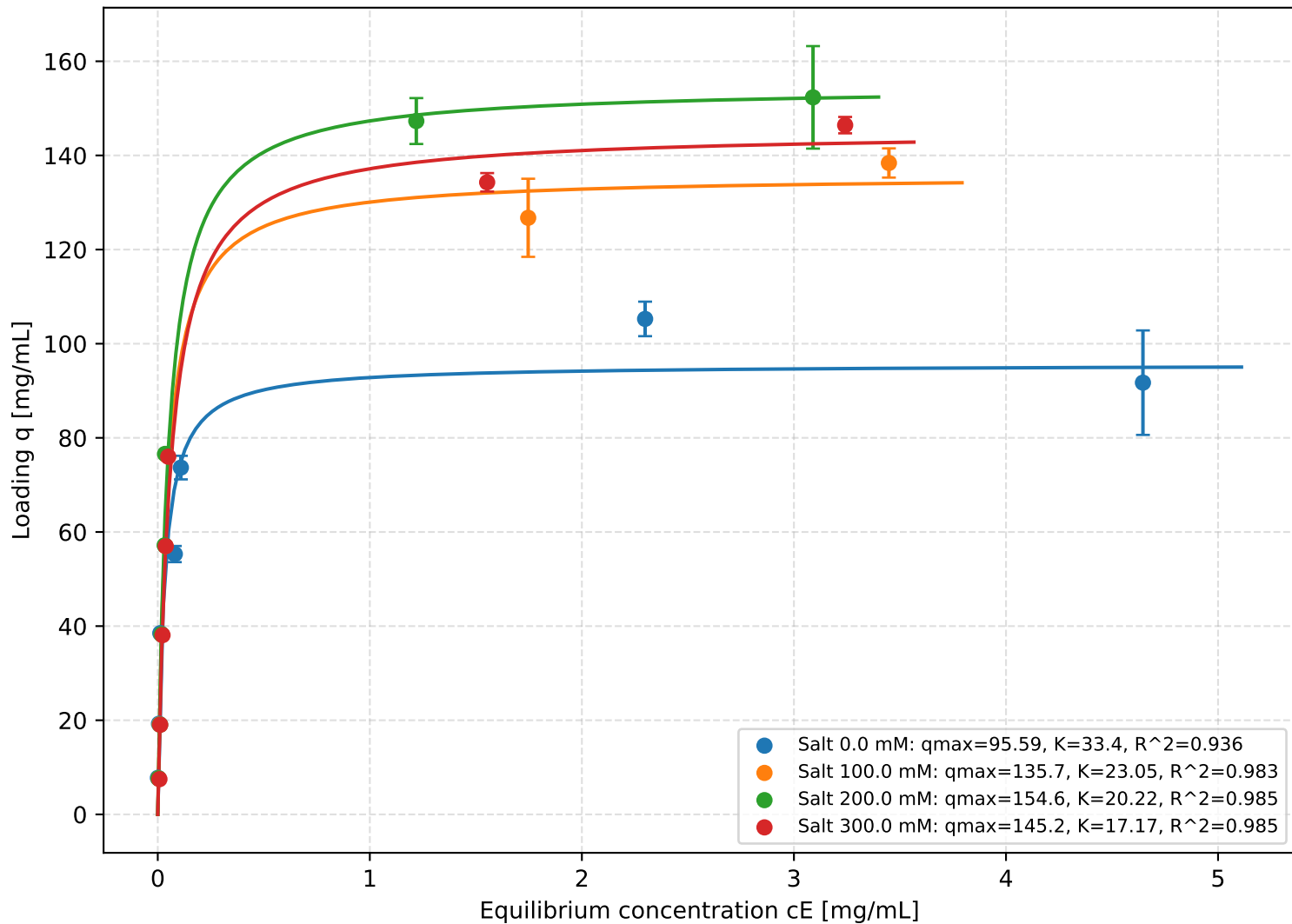
Loading Isotherms - Experiment 5025 at 280 nm
